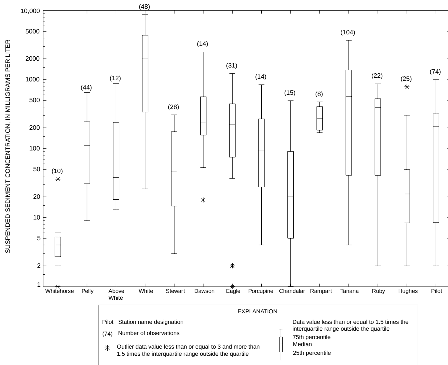
Figure 26. Boxplots of suspended-sediment concentrations at 14 sites in the Yukon River Basin.
