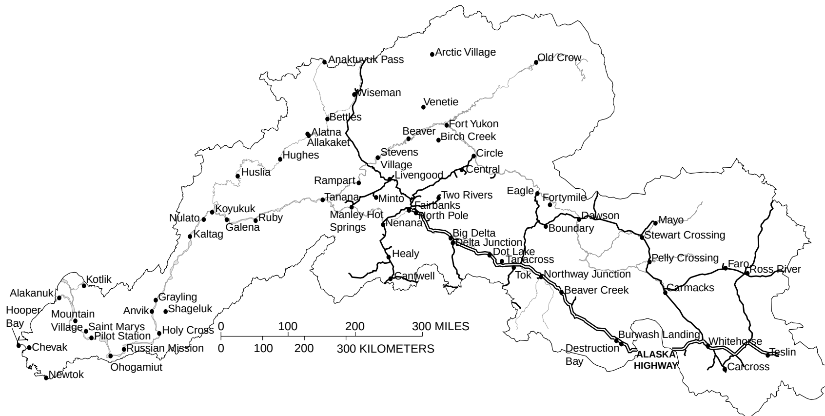
Figure 5B. Roads and towns in the Yukon River Basin.
