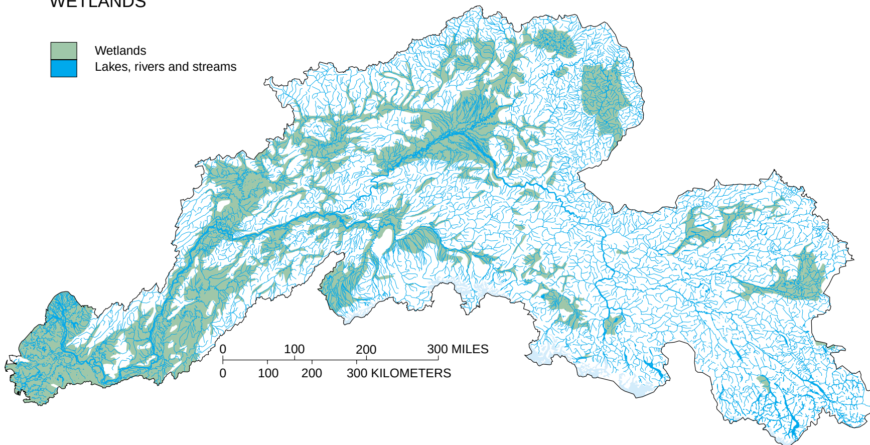
Figure 14. Wetland areas of the Yukon River Basin (modified from Fretwell and others, 1996).
