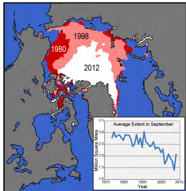
Minimum annual sea ice extent has been decreasing. Source: NSIDC 2012.
