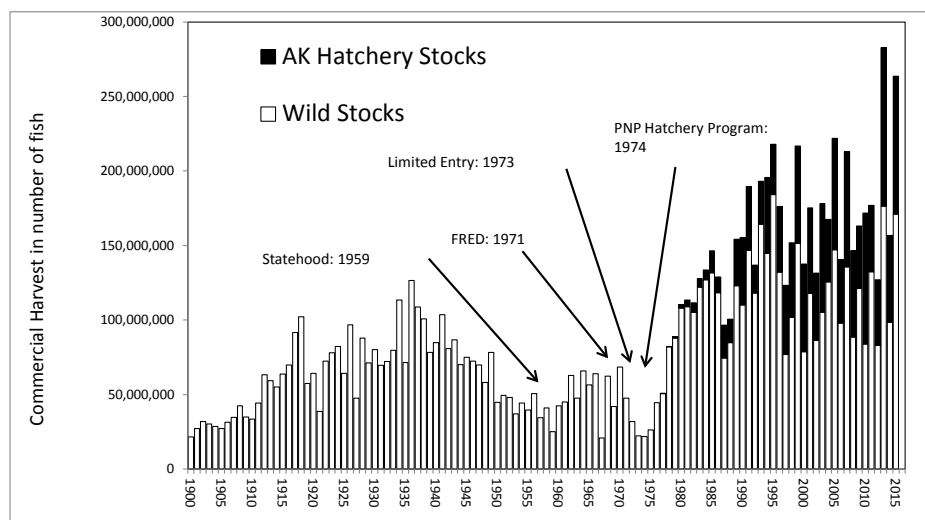
Commercial salmon harvest in Alaska, 1900-2015. Alaska salmon stocks rebounded dramatically after the 1976-1977 regime shift. Source: Stopha 2015.
