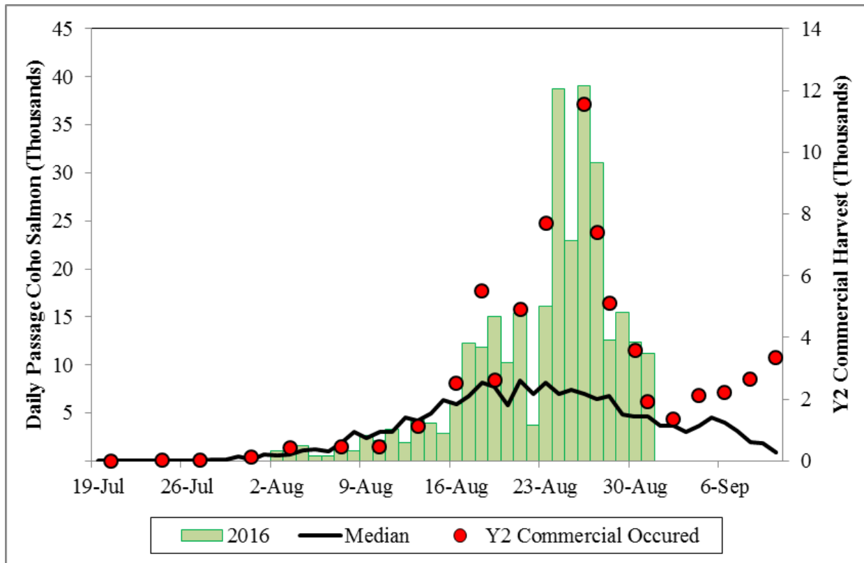
Figure 3.—Run reconstructed daily Yukon River mainstem sonar (Pilot Station) passage estimates attributed to coho salmon with commercial periods and harvest indicated 2016, compared to historical median.
